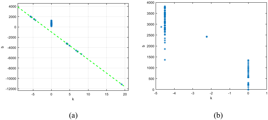
Fig. 7. Points in parameter space after Hough transformation (a) points in parameter space of original image; (b) points in parameter space of affine rectified image. (Color figure online)
