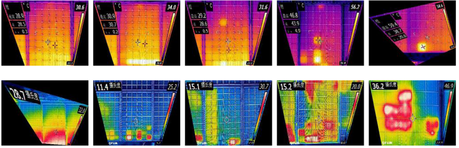
Fig. 9. The rectified IR images of PV modules
