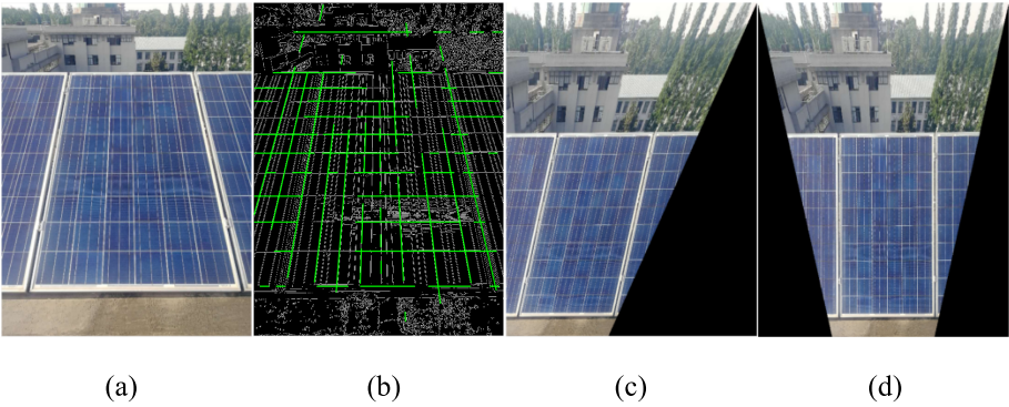
Fig. 6. Removing projective distortion of photovoltaic modules (a) original image; (b) lines detection by Hough transformation; (c) affine rectification; (d) recovery of right angles.
