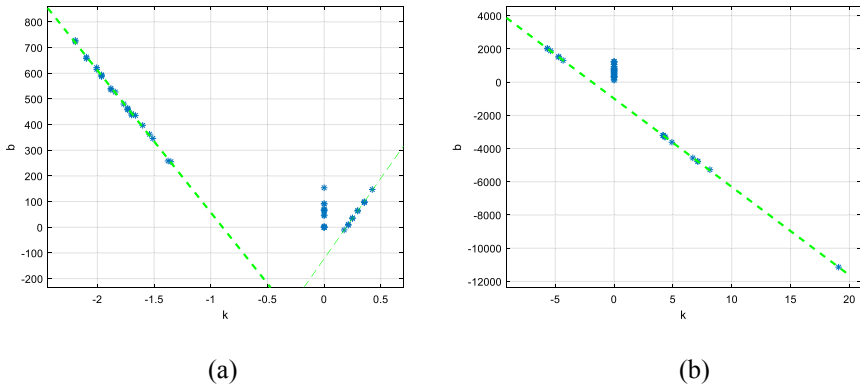
Fig. 2. Points in parameter space after Hough transformation (a) two lines in parameter space correspond to two vanishing points in image space; (b) a single line in parameter space corresponds to a single vanishing point in image space.
