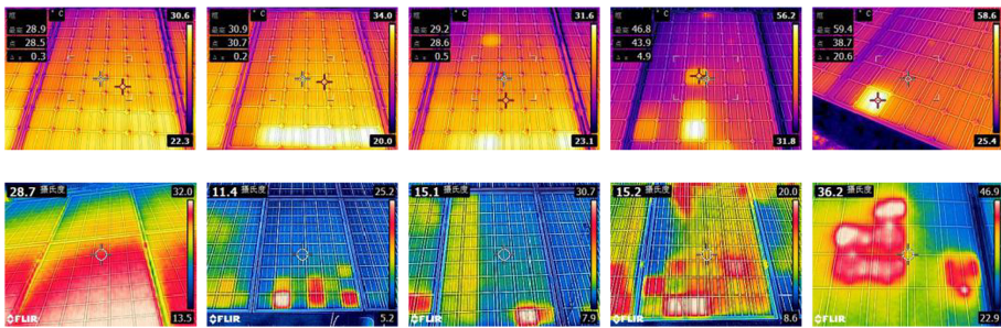
Fig. 5. Infrared images of photovoltaic modules
